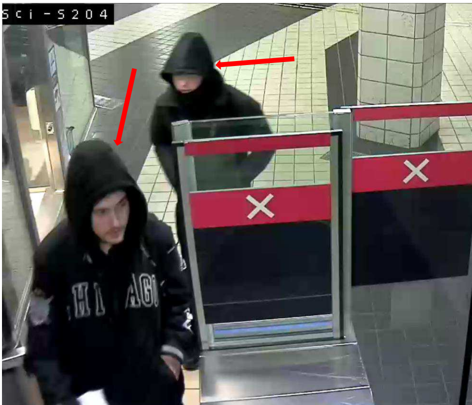
Sci-S204, 21:11:42
