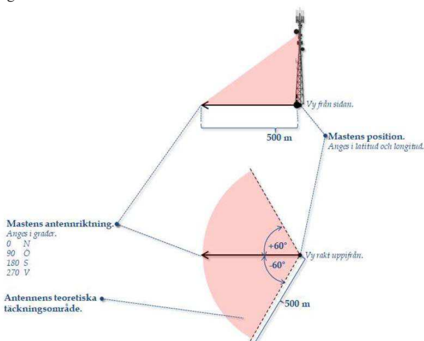
Figur 5. Basstation.
