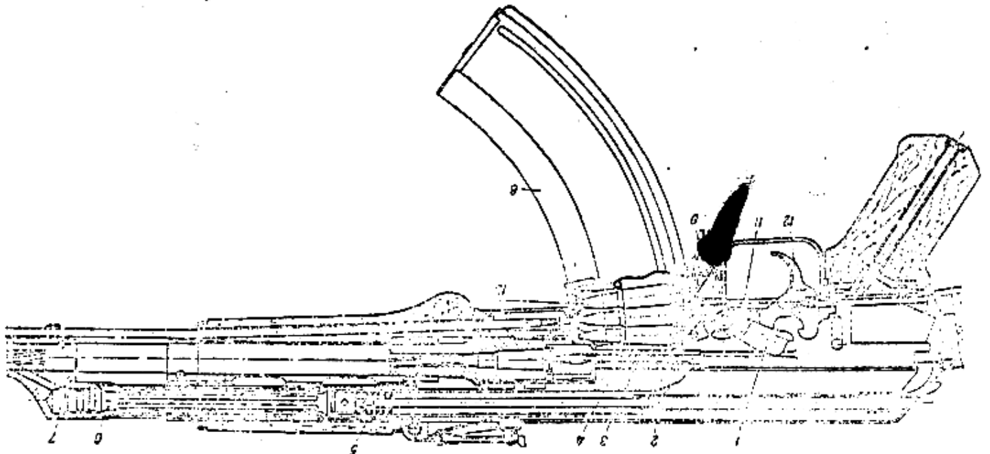
Figure 63. Position of parts after loading and before firing.
