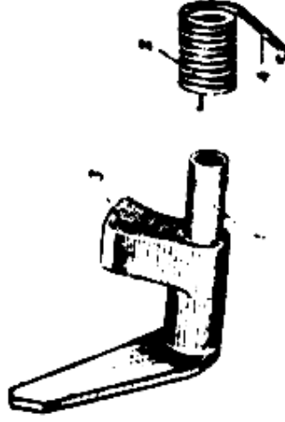
Figure 40. Full automatic sear with stamped receiver.
