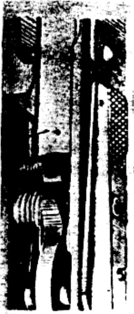
Figure 41. Fastening of long end of full automatic sear spring in rifle with stamped receiver.
