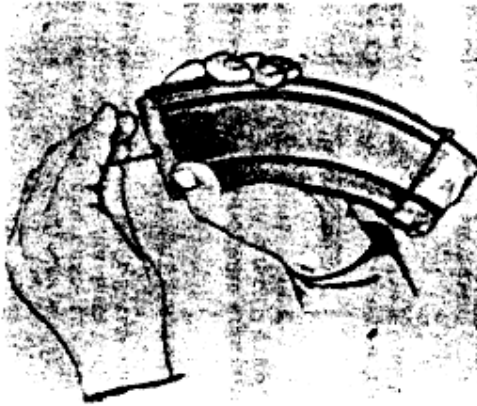
Figure 82. Removing the cover plate from the magazine.
