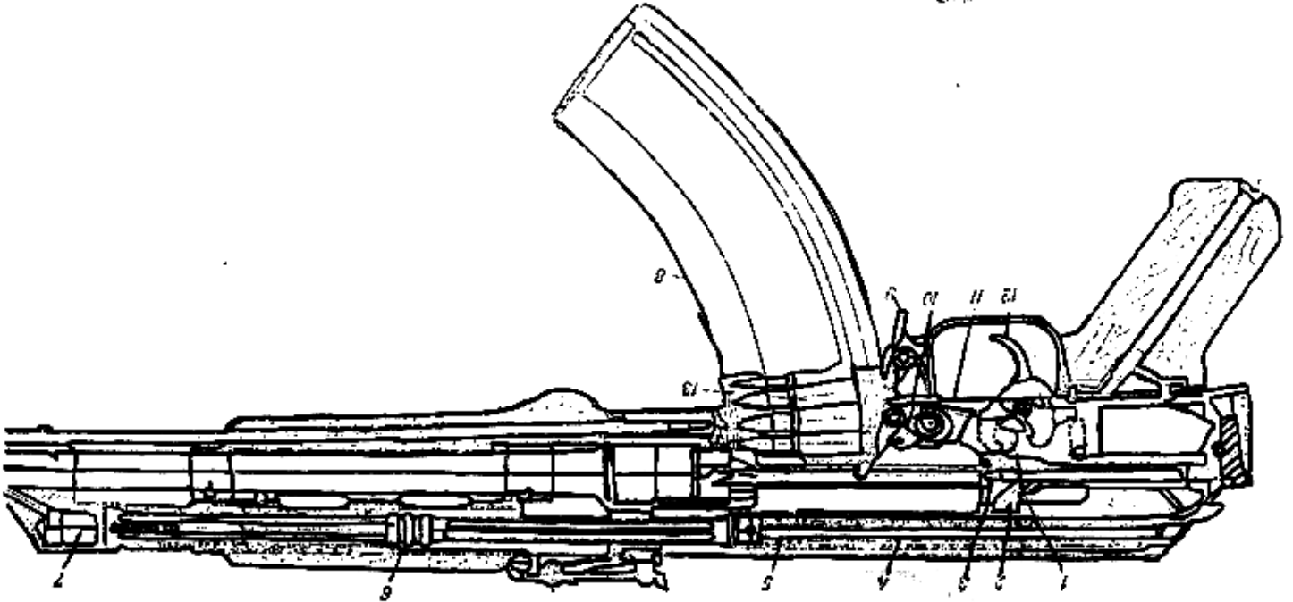
Figure 62. Position of parts with operating rod in extreme rear position.
