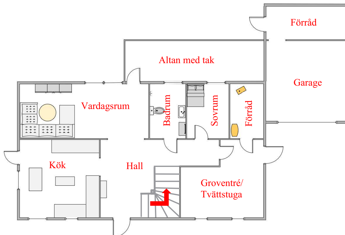
Figur 4. Markplan.
